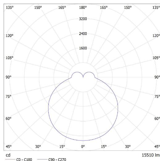
Lucis IR.L14.1500M.1 IZAR R MAX LED / LDC (Polar)
